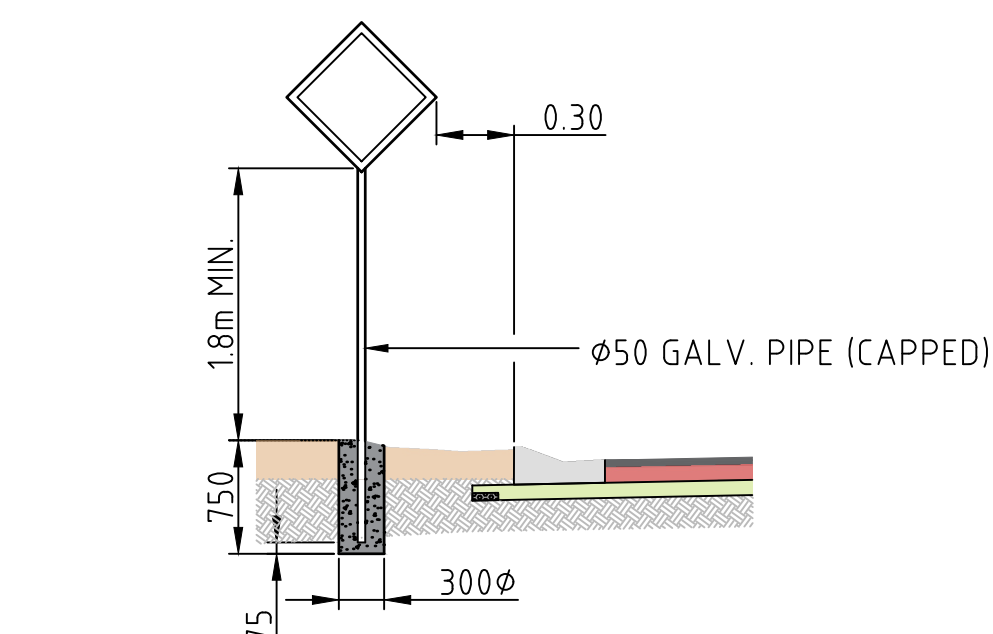
ROAD EDGE SIGN POST TYPICAL DETAIL
