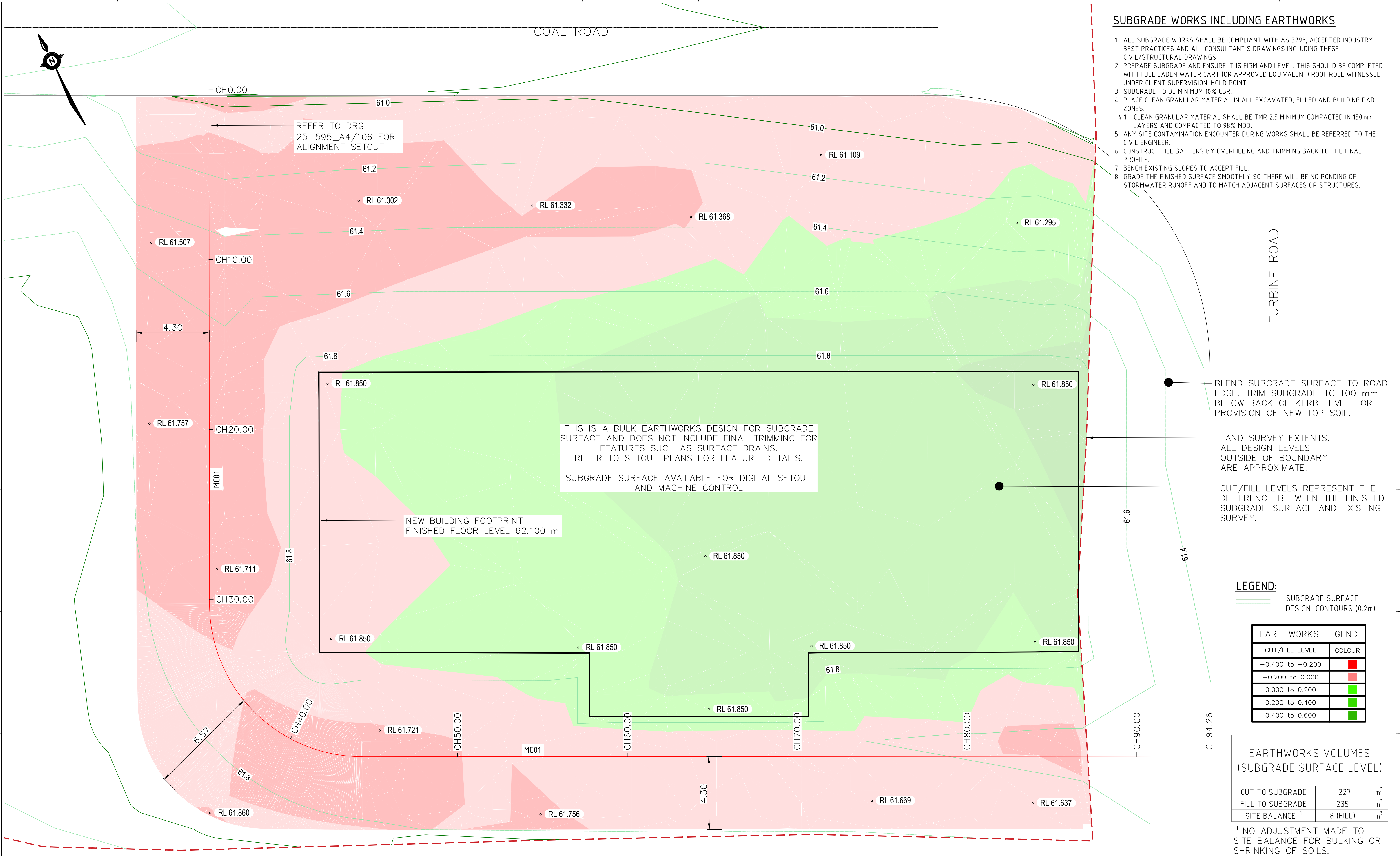
EARTHWORKS CUT/FILL PLAN SCALE 1:100
