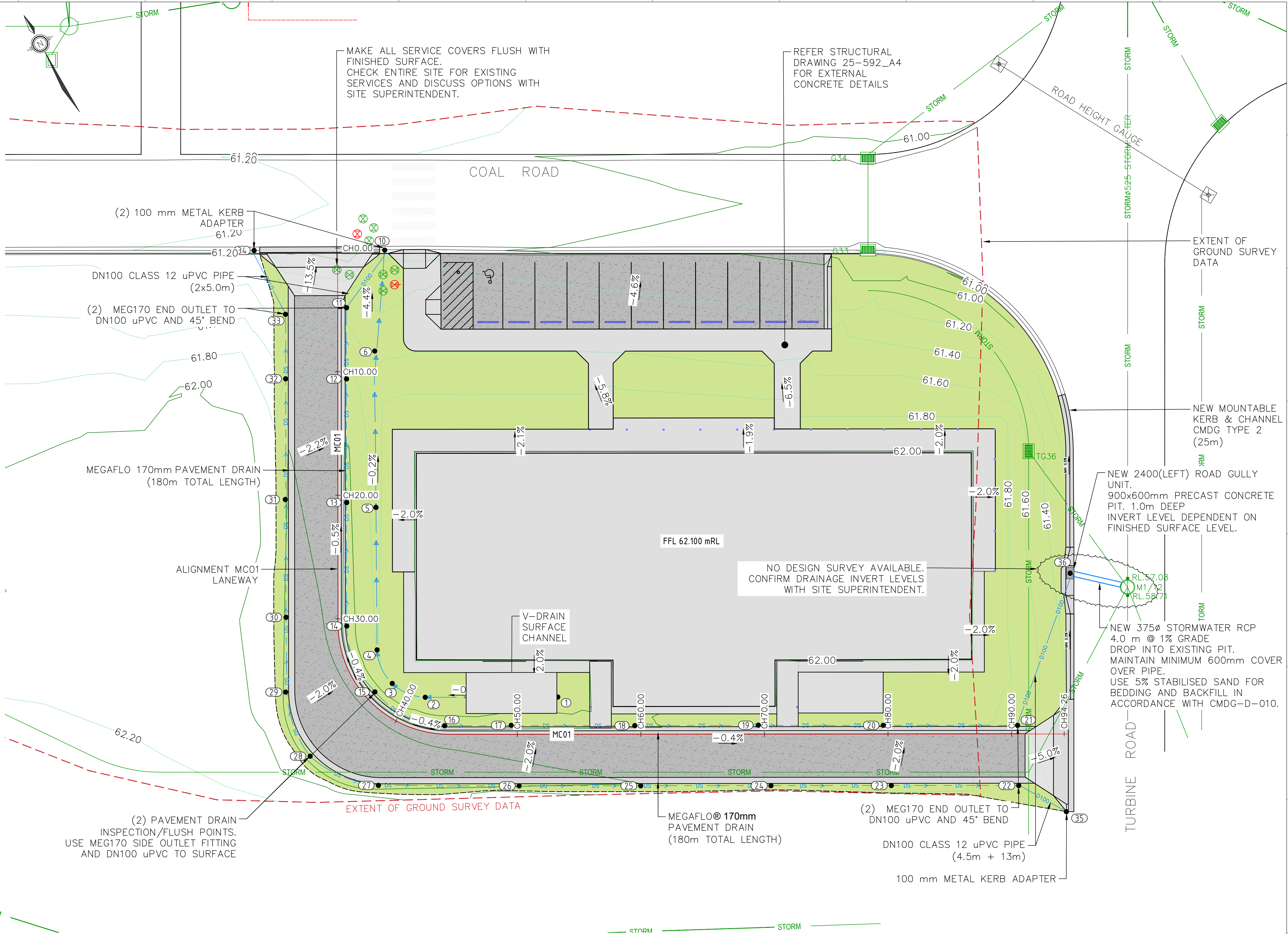
DRAINAGE DESIGN LAYOUT SCALE 1:150
