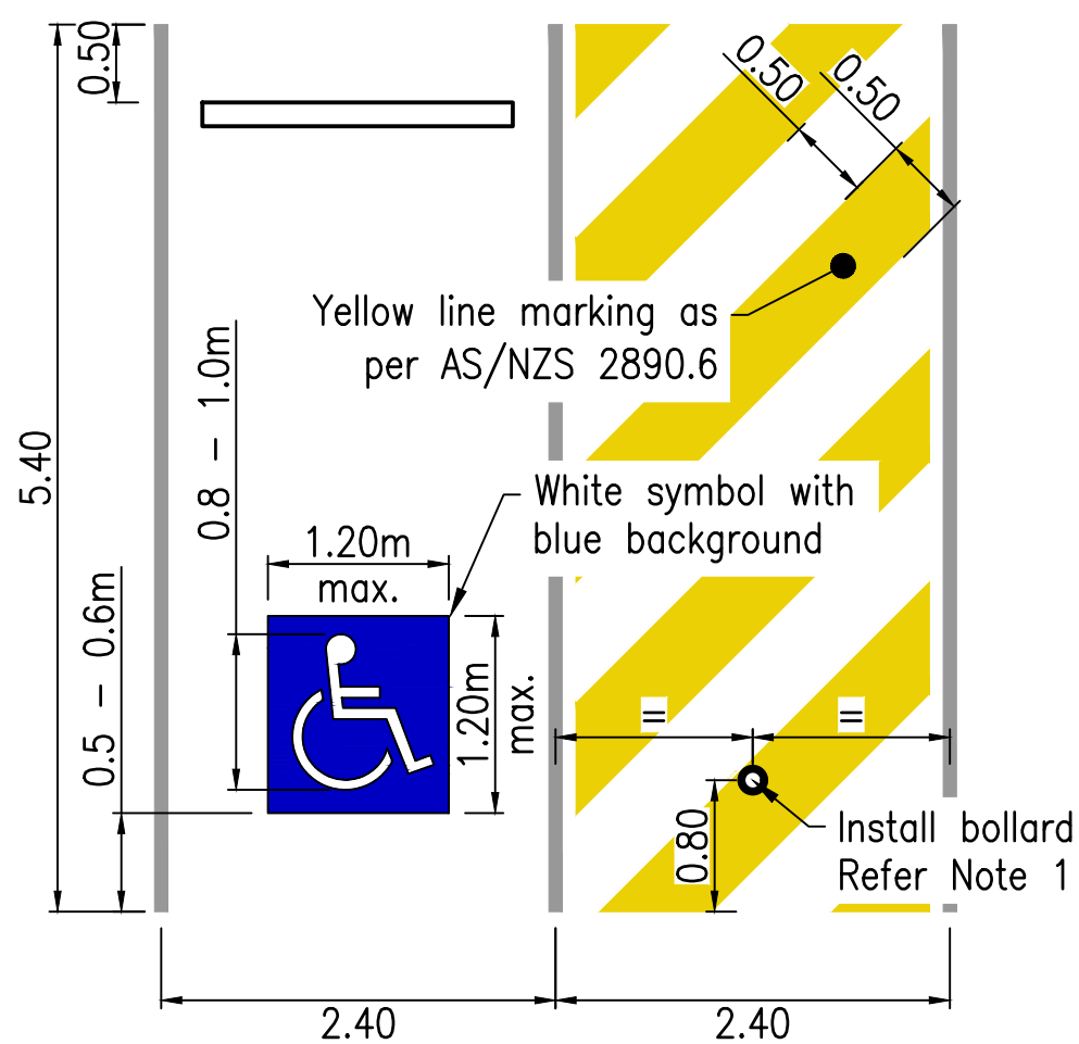
ACCESSIBLE PARKING BAY TYPICAL DETAIL SCALE 1:50
